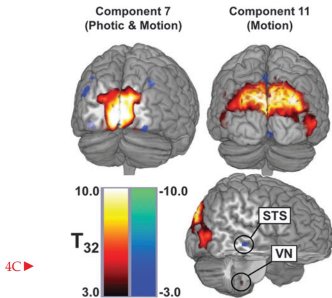
FIG. 5. Spatial distributions of the two networks identified by multiple regression analysis. These maps were produced by masking the spatial t -tests with the z-scored image. Component 7 (left) was modulated by both visual tasks and localizes to the posterior occipital lobe. Component 11 (right) was modulated only by Motion and includes multiple visual association cortices, the superior temporal sulcus (STS), which is part of the multisensory processing network, and a region within the brainstem that appears to be the vestibular nucleus (VN). This view does not present all active regions for each network but does show the largest areas and those consistent with previous studies using optic flow.
